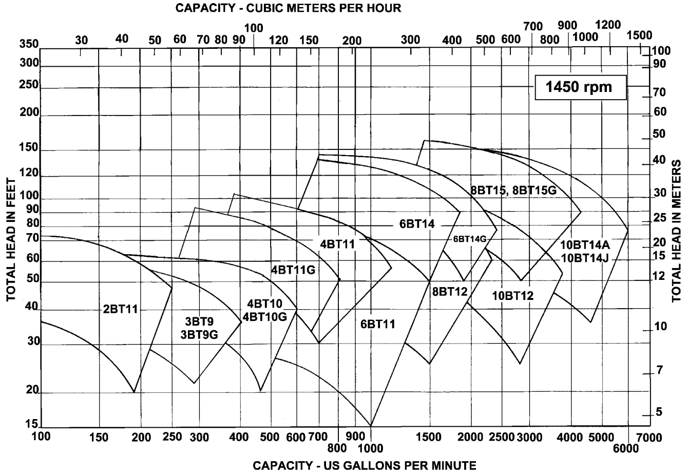
Area Bound Performance Curves 1450 Rpm
