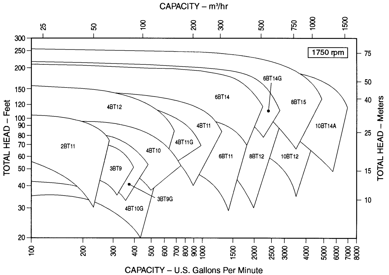
Area Bound Performance Curves 1750 Rpm
