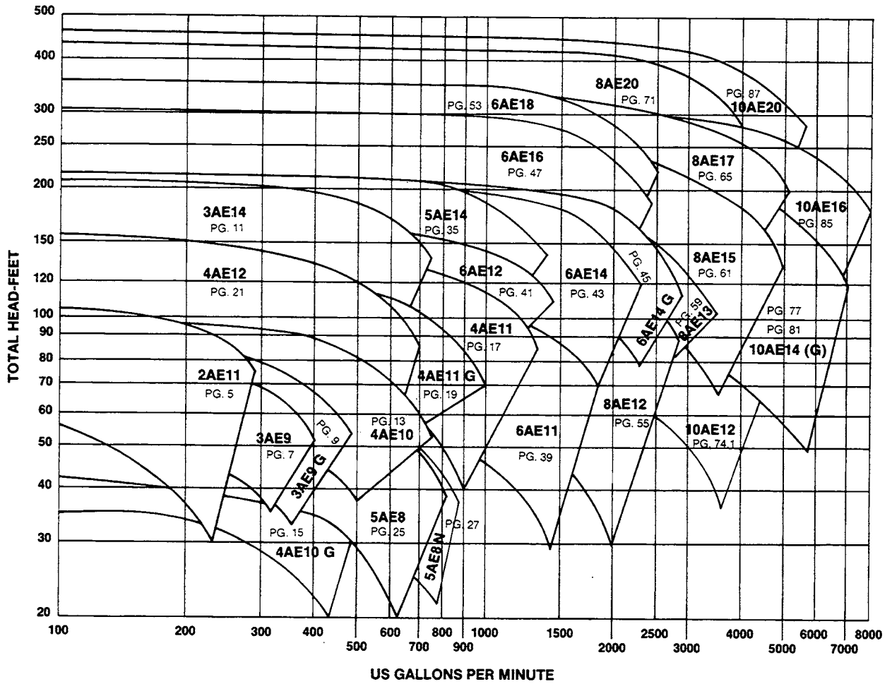
AREA BOUND CURVES* 1750 NOMINAL RPM
