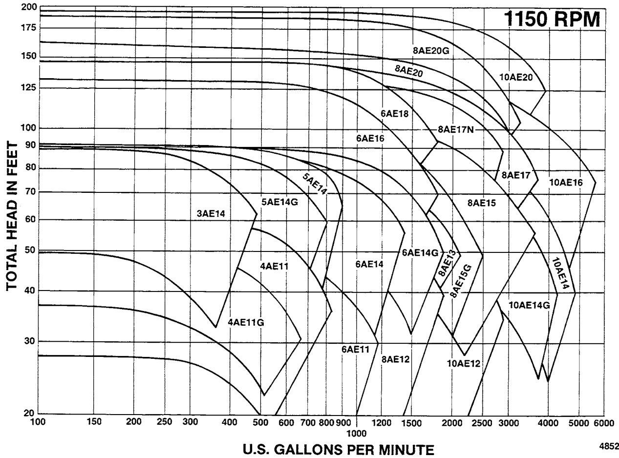
Area Bound Curves* 1150 Nominal Rpm
