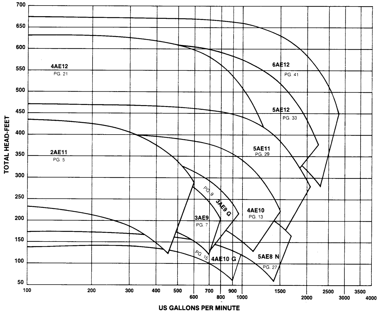
AREA BOUND CURVES* 3550 NOMINAL RPM
