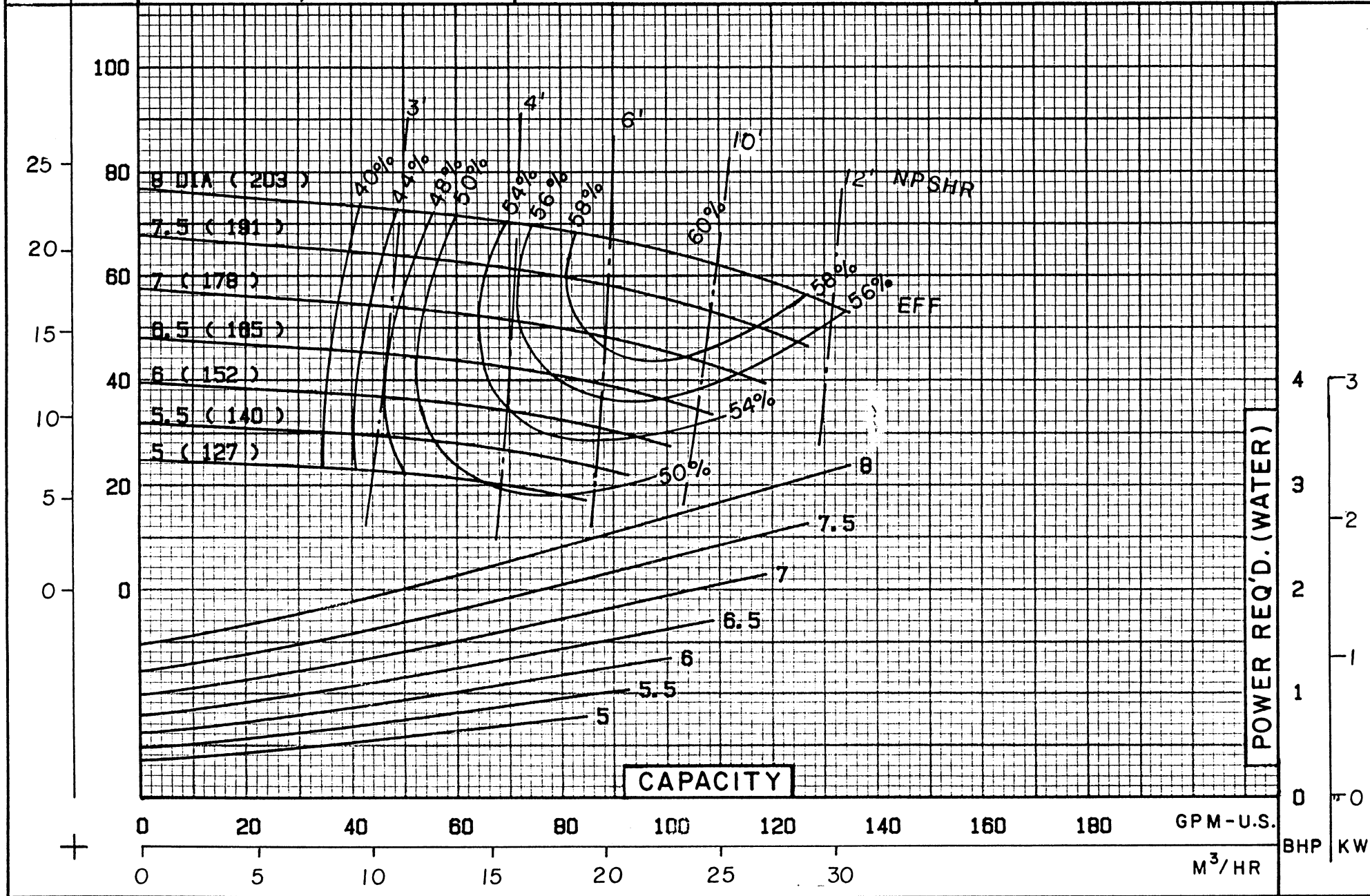
CURVE NO. V-AB8-17A
