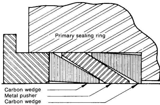
FIGURE 3. Compound carbon wedge secondary seal
