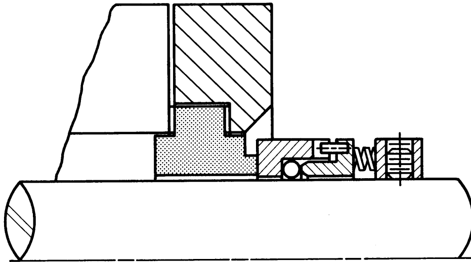
FIGURE 10. Single outside seal
