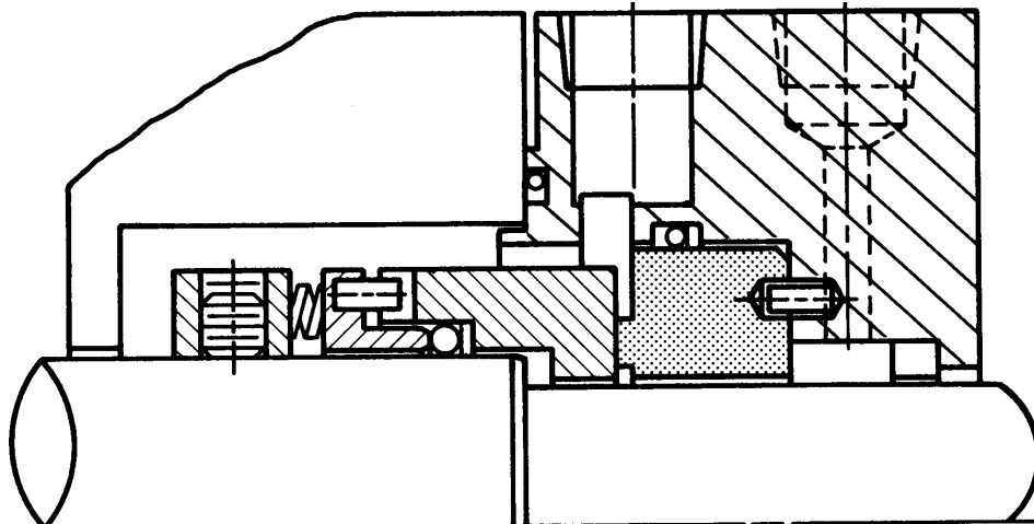
FIGURE 8. High pressure seal
