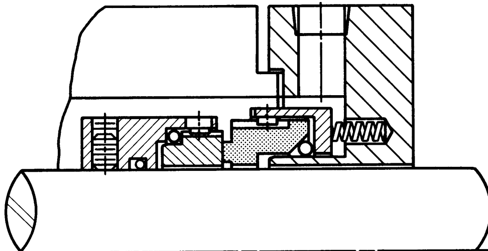
FIGURE 9. Typical high speed seal
