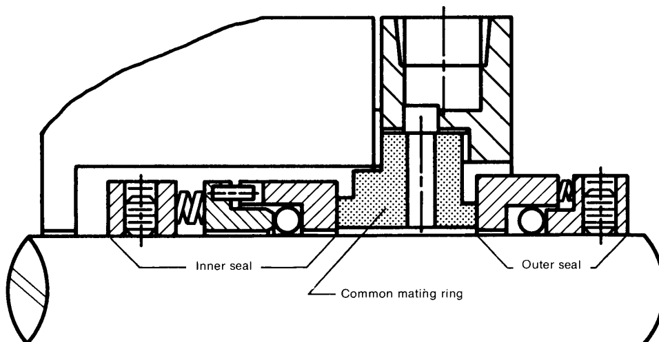
FIGURE 13. Double inside-outside seal
