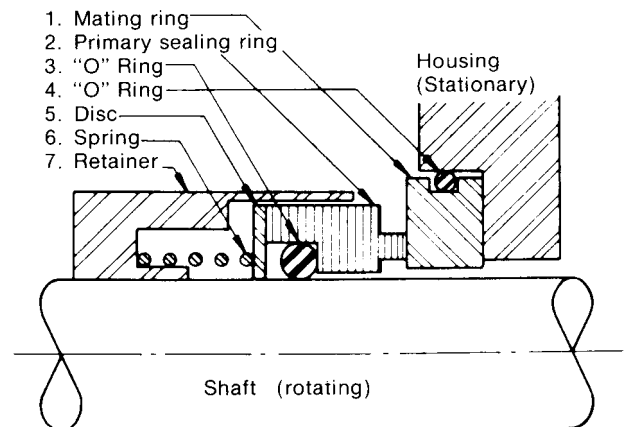
FIGURE 1. Mechanical end face seal
