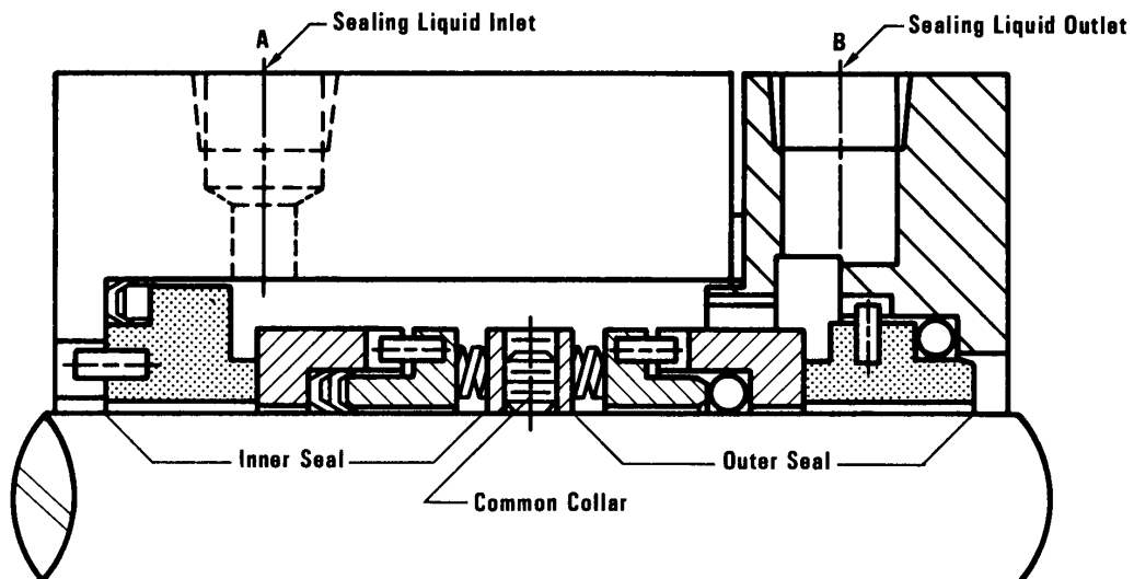
FIGURE 11. Double inside seal
