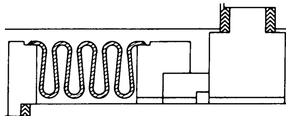
E: Formed metal bellows seal
