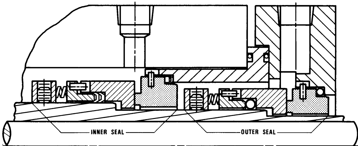
FIGURE 12. Double tandem seal
