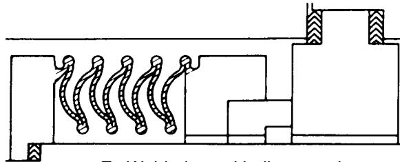
F: Welded metal bellows seal
