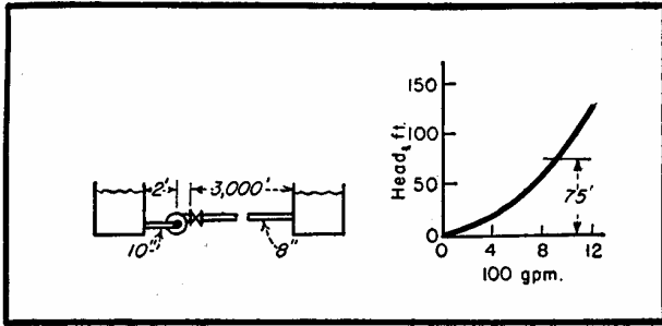
NO LIFT—ALL FRICTION HEAD
