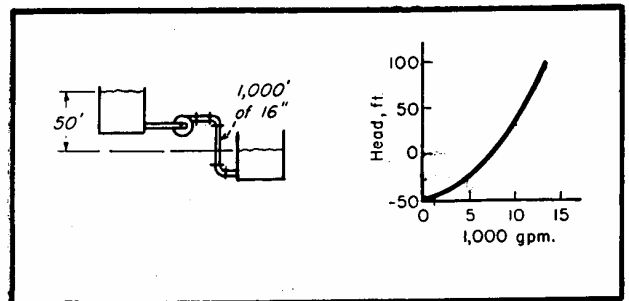
NEGATIVE LIFT (GRAVITY HEAD)
