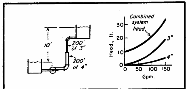
TWO DIFFERENT PIPE SIZES
