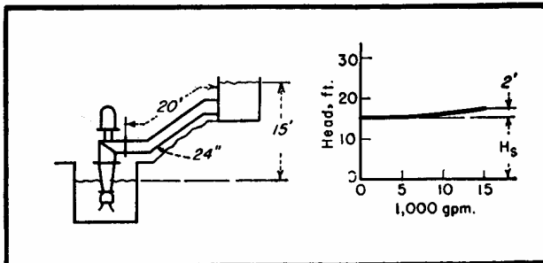
MOSTLY LIFT—LITTLE FRICTION HEAD
