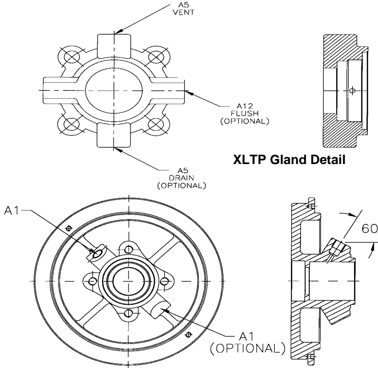
XLTP Stuffing Box Detail
