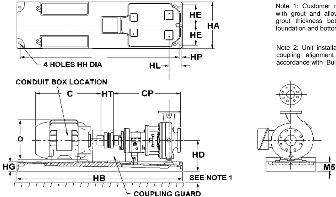
Dimensions apply only to Pump Sizes 4x6-10, 1-1/2x3-13, 2x3-13, 3x4-13, 4x6-13
