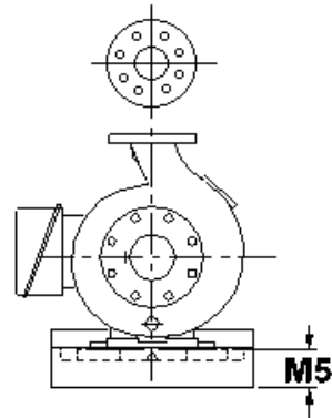
Dimensions apply only to Pump Sizes 2x3-6, 2x3-8, 3x4-8, 3x4-8G, 1x2-10, 1-1/2x2-10, 2x3-10, 3x4-10
