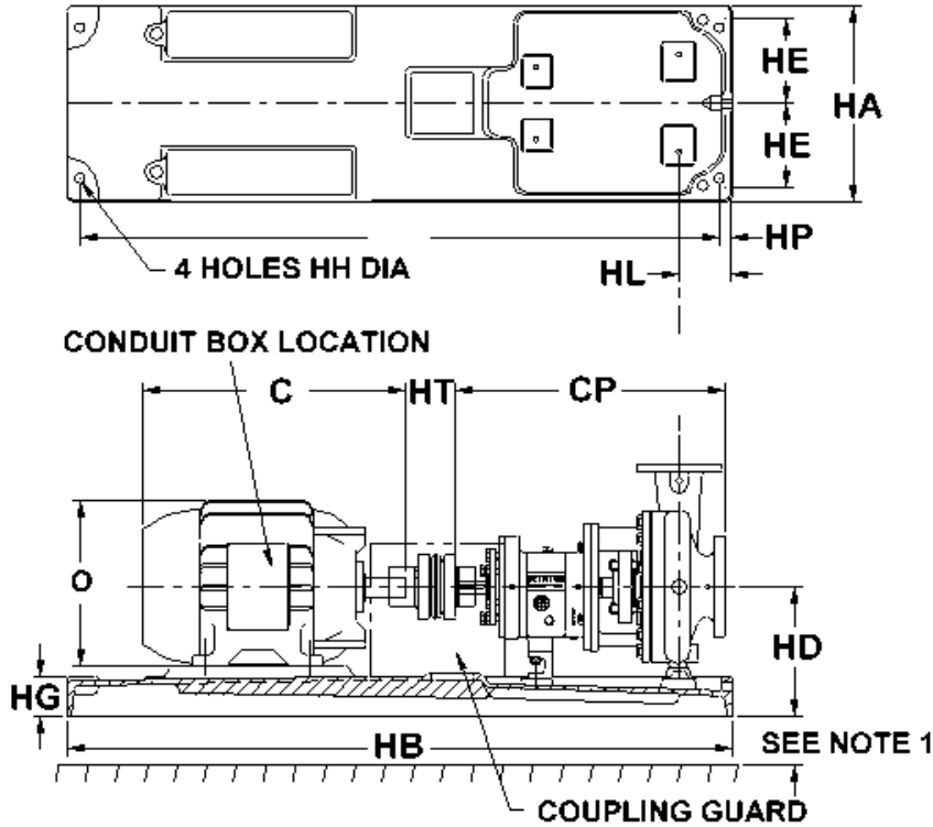
Dimensions apply only to Pump Sizes 2x3-6, 2x3-8, 3x4-8, 3x4-8G, 1x2-10, 1-1/2x2-10, 2x3-10, 3x4-10
