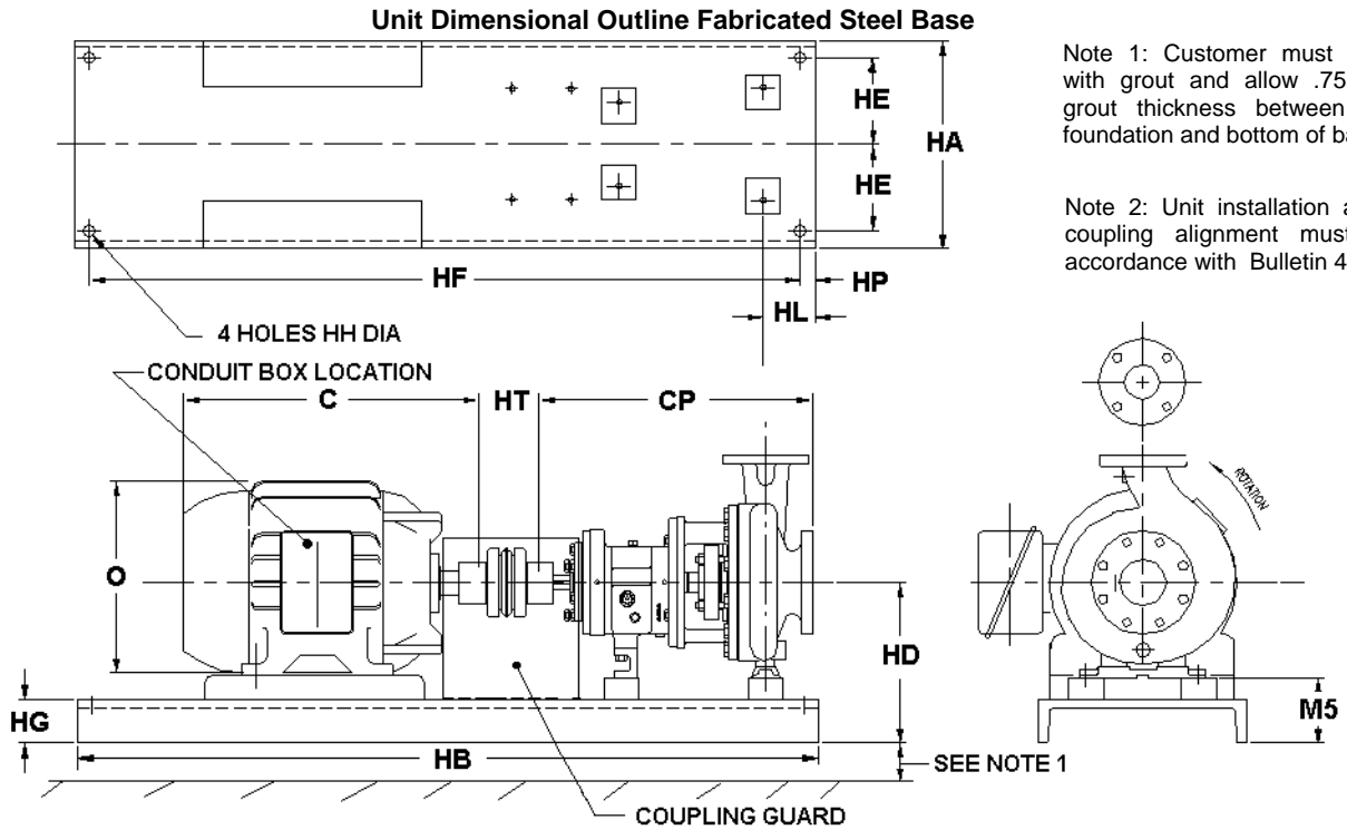
Dimensions apply only to Pump Sizes 4x6-10, 1-1/2x3-13, 2x3-13, 3x4-13, 4x6-13
